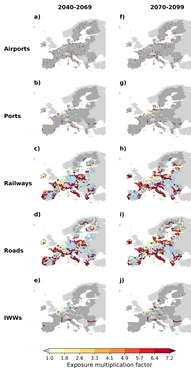
Figure A7. Maps of multi-model ensemble median exposure multiplication factors of the TEN-T by mode (rows) to floods by the middle (2040–2069) and the end of the century (2070–2099) (columns) relative to historical climate conditions (1980–2009) under a high emission scenario (RCP8.5). The multi-model ensemble median is computed across all available combinations of impacts models and GCMs.
