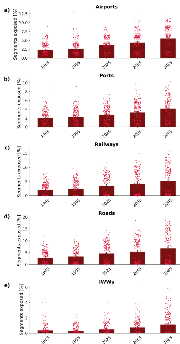
Figure 10. Percentage of European transport elements exposed to wildfires over time under a medium-high emissions scenario (RCP6.0). The bar plot shows the mean percentage of exposed transport elements computed by pooling all annual values across all GCM-impact model simulations within each 30-year window. The black error bar denotes the 95 % bootstrap confidence intervals for the mean. Each dot represents the percentage of exposed segments for a single GCM-impact model pair, based on the number of transport elements in each grid cell projected to experience exposure. The year on the x-axis denotes the central year of a 30-year window (e.g., 1965 represents 1950–1979).
