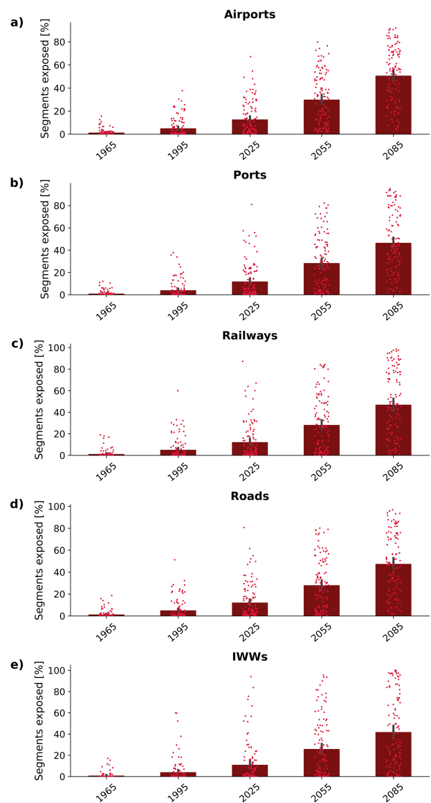
Figure 8. Percentage of European transport elements exposed to heatwaves over time under a medium-high emissions scenario (RCP6.0). The bar plot shows the mean percentage of exposed transport elements computed by pooling all annual values across all GCM-impact model simulations within each 30-year window. The black error bar denotes the 95 % bootstrap confidence intervals for the mean. Each dot represents the percentage of exposed segments for a single GCM-impact model pair, based on the number of transport elements in each grid cell projected to experience exposure. The year on the x -axis denotes the central year of a 30-year window (e.g., 1965 represents 1950–1979).
